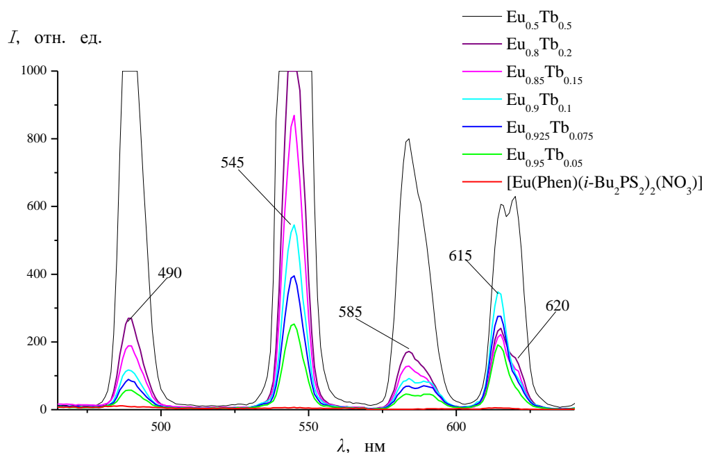
Рис. 68. Спектры ФЛ ( \lambda_{возб} = 330 нм) комплекса [\text{Eu}(\text{Phen})(i\text{-Bu}_2\text{PS}_2)_2(\text{NO}_3)] и твёрдых фаз двойной системы [\text{Eu}(\text{Phen})(i\text{-Bu}_2\text{PS}_2)_2(\text{NO}_3)] – [\text{Tb}(\text{Phen})(i\text{-Bu}_2\text{PS}_2)_2(\text{NO}_3)] ( \text{Eu}_{0.5}\text{Tb}_{0.5} , \text{Eu}_{0.8}\text{Tb}_{0.2} , \text{Eu}_{0.85}\text{Tb}_{0.15} , \text{Eu}_{0.9}\text{Tb}_{0.1} , \text{Eu}_{0.925}\text{Tb}_{0.075} и \text{Eu}_{0.95}\text{Tb}_{0.05} )
